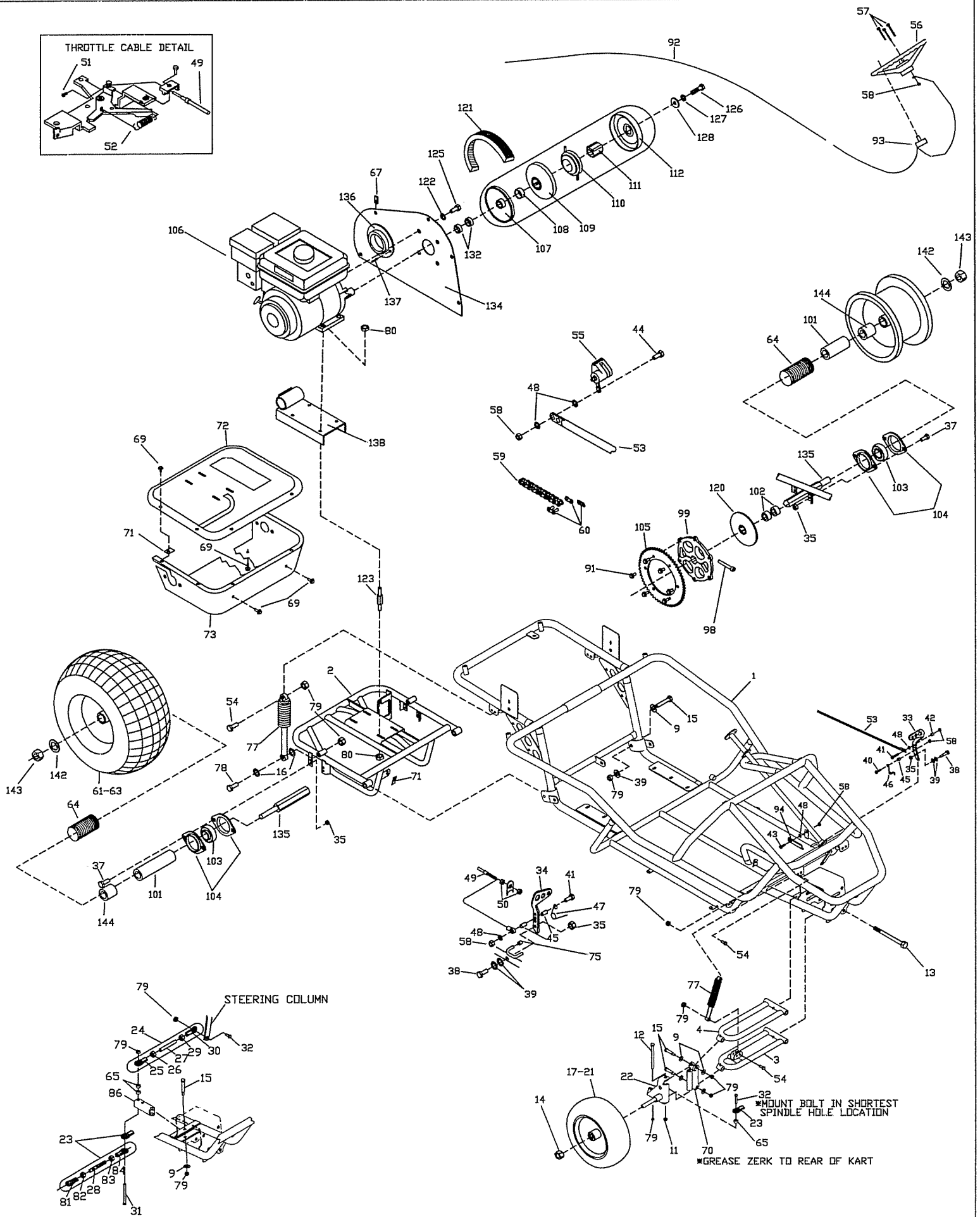
STEERING DETAIL
